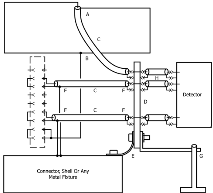
FIG. 1 Equipment Setup for Amplitude Sensitivity Measurement
