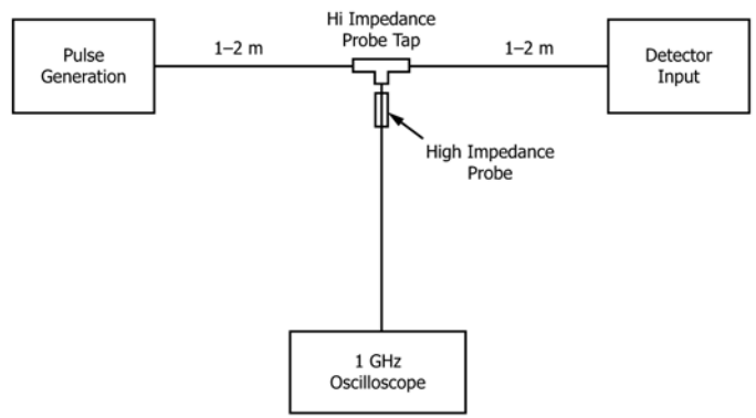
FIG. 1 Equipment Setup for Amplitude Sensitivity Measurement
